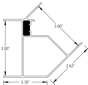
7906A 3" 45° Corner Channel
