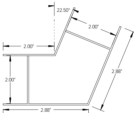
7719A 2" 22.5° Corner Channel
