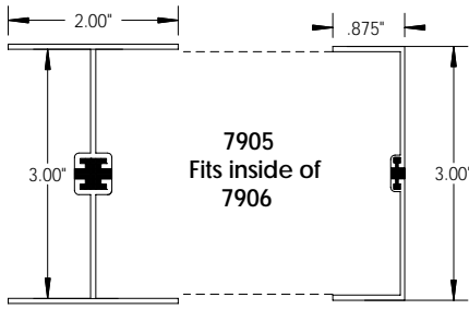
7903 3" H Channel
