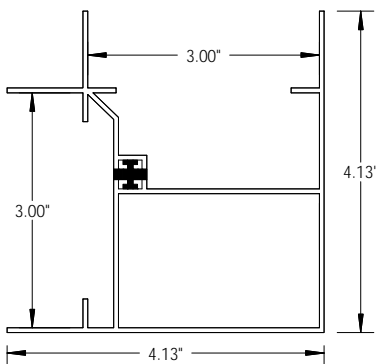
7906 3" Corner Channel
