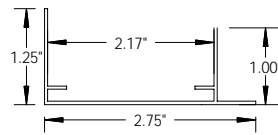
7712 2" F Base Channel
