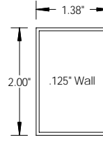
77107 2" Extruded Column Insert
