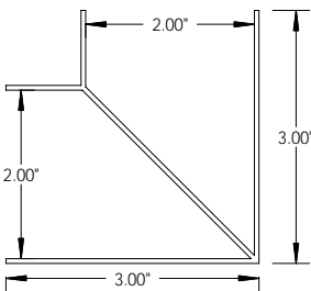
7719 2" Corner Channel
