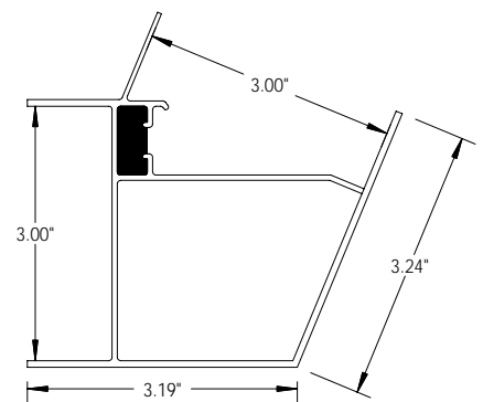
7906B 3" 22.5° Corner Channel
